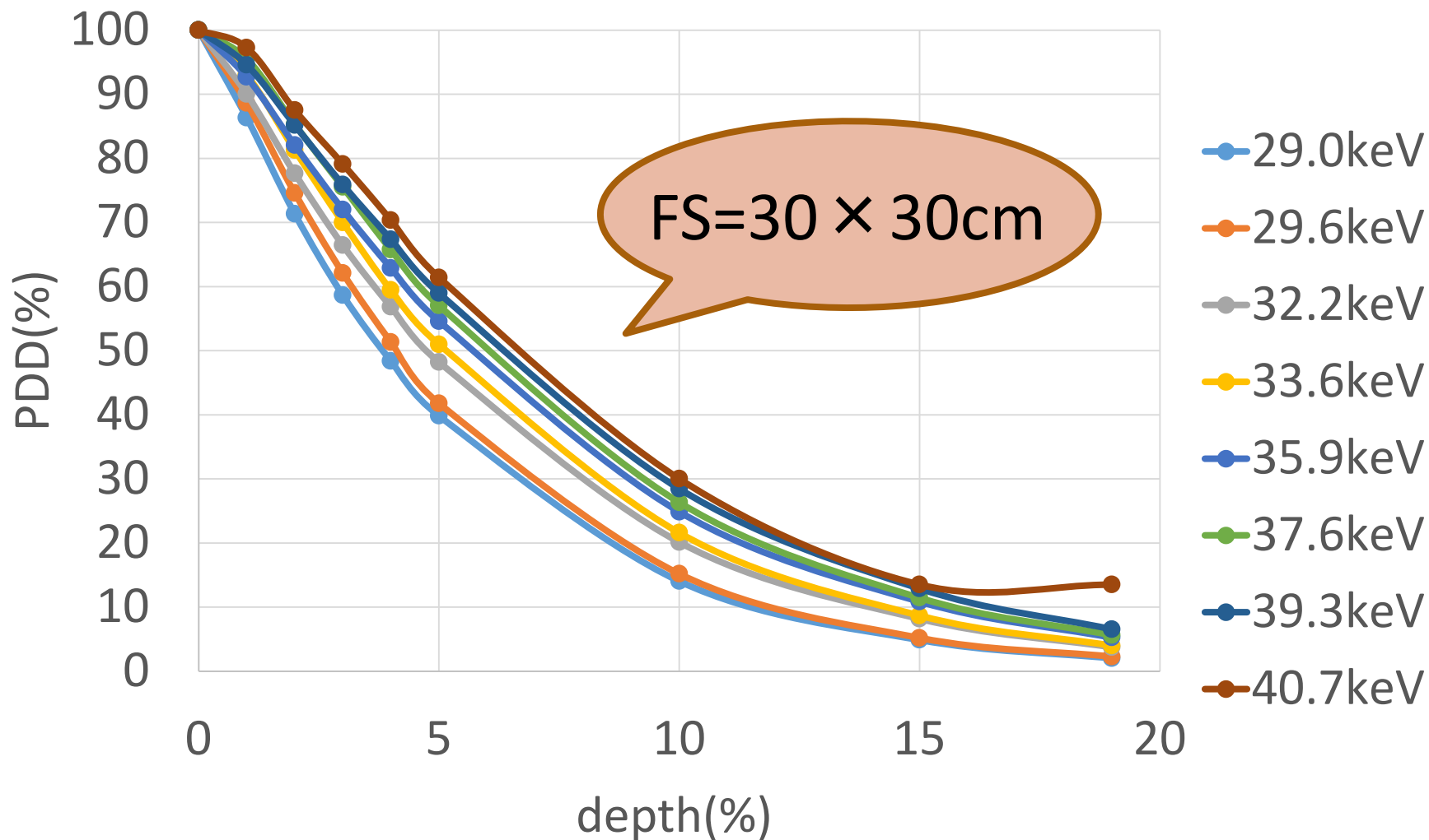
Fig.3 The percentage depth dose curve (FS=30 × 30cm)
