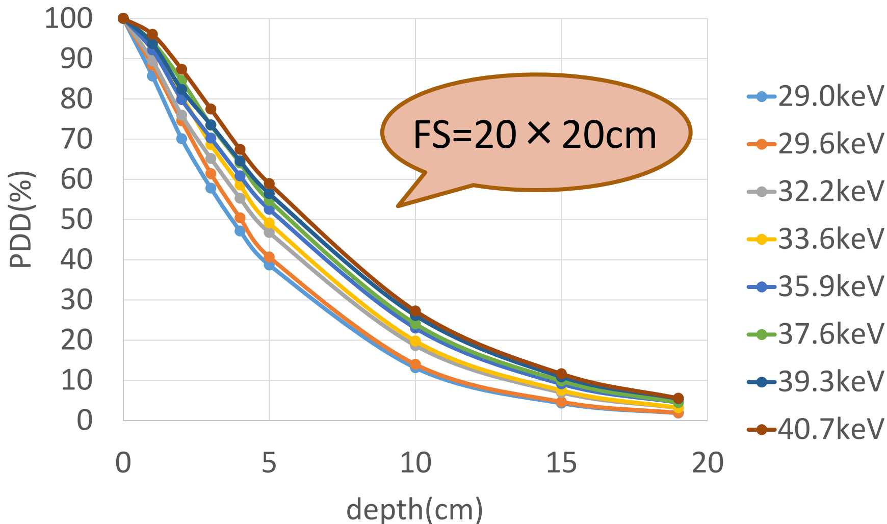
Fig.2 The percentage depth dose curve (FS=20 × 20cm)
