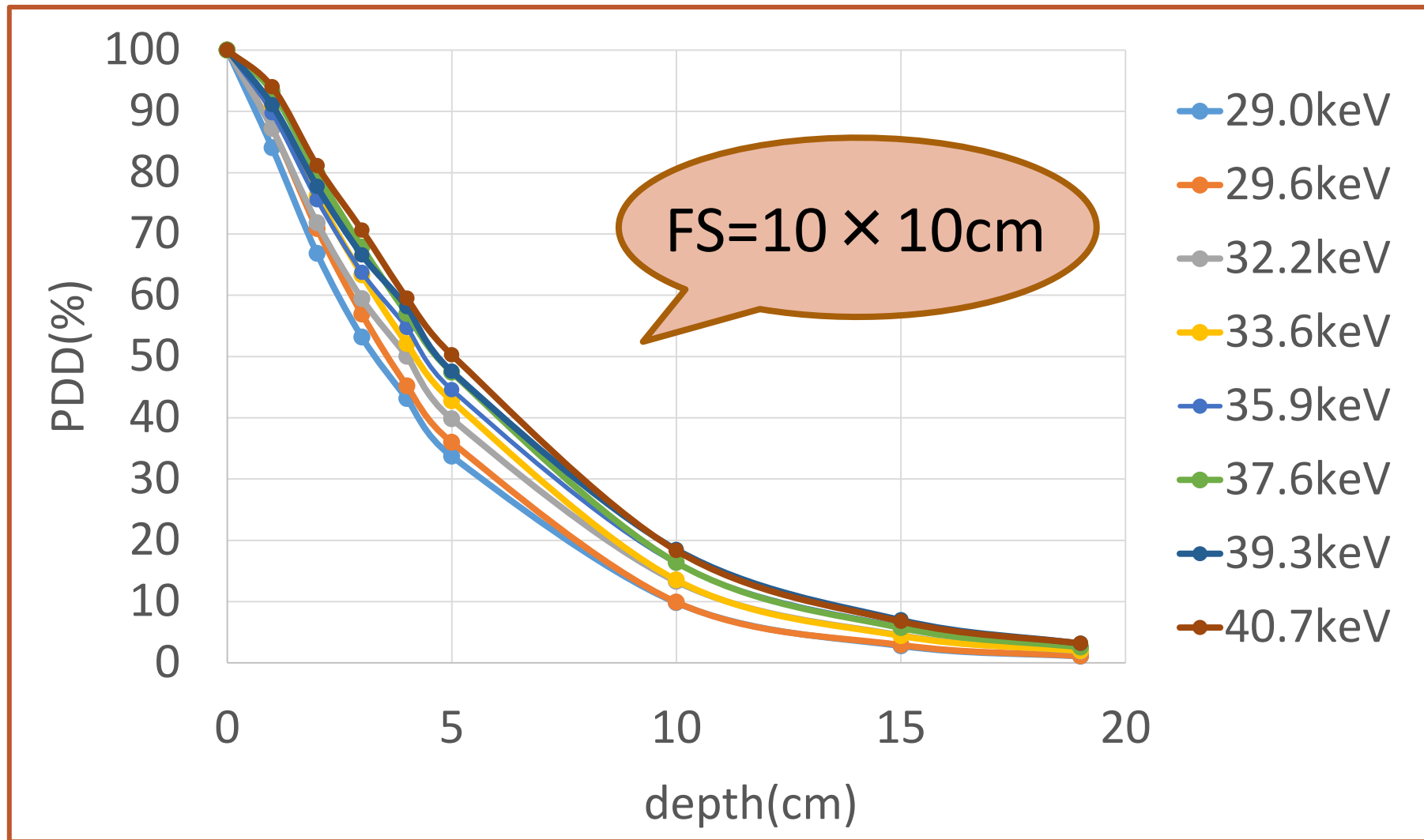
Fig.1 The percentage depth dose curve (FS=10x10cm)
